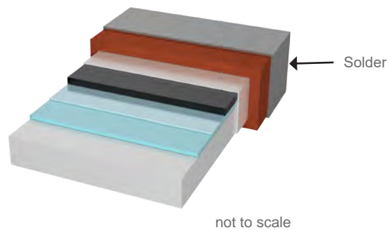
Fig. 6: Architecture of the TPL5000-series
