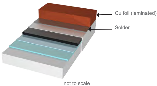
Fig. 4: Architecture of the TPL2000-series
