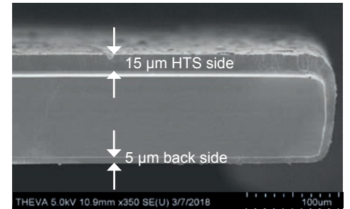
SEM cross section of PVD copper coating
